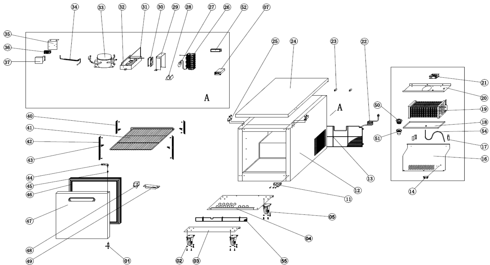
EXPLODE OF KCHUC27R-32
